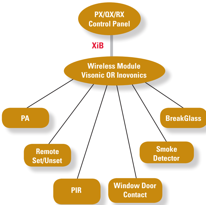
Transmitters (TXs)... Visonic or Inovonics
