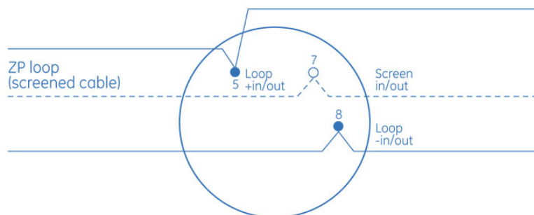
ZP7-SB1 / ZP7-RB1 Sensor base
